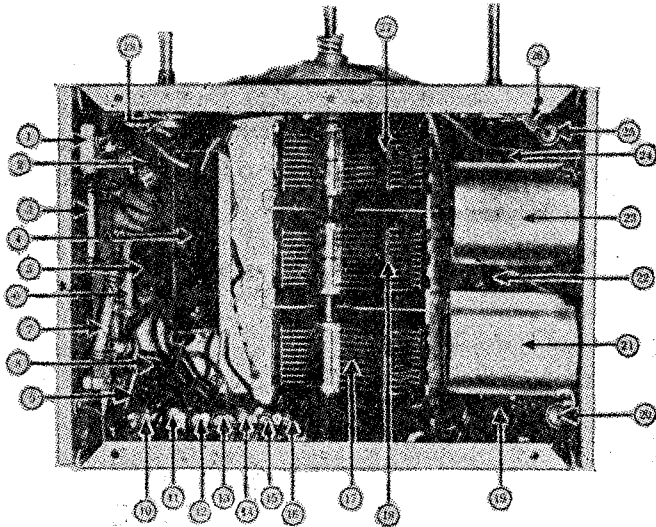
Interior View of Model 55 Chassis
